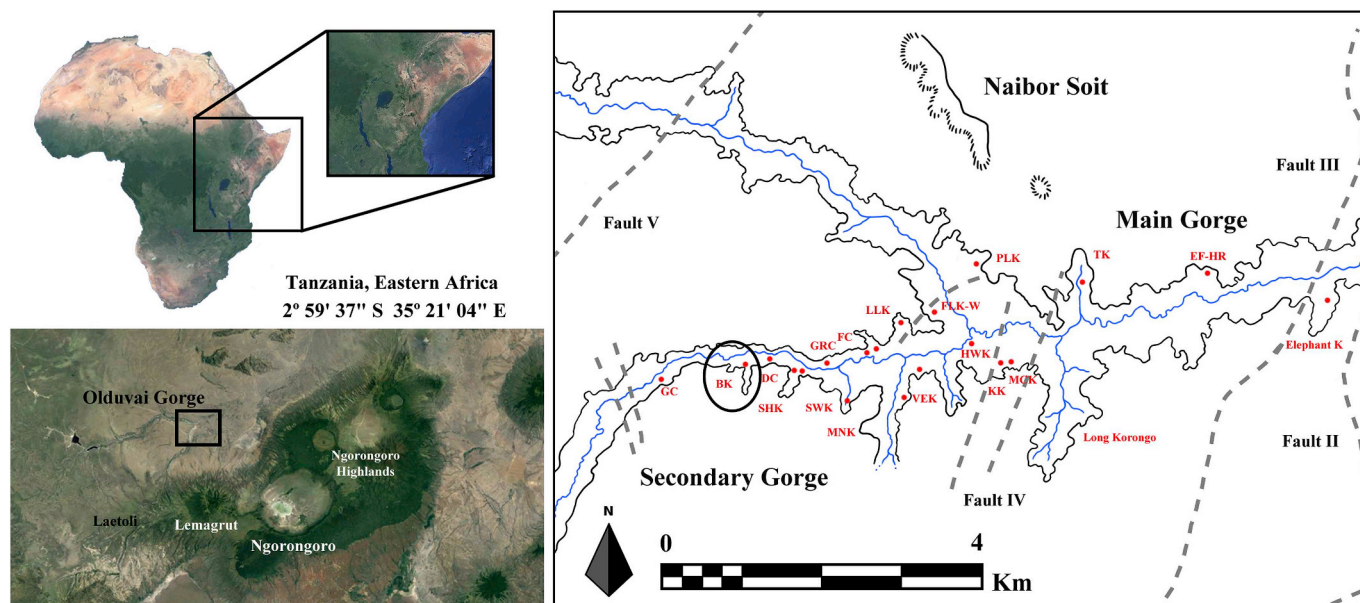
Fig. 1. Geographic location of the Olduvai Gorge (Left) and the site of BK in relation to other key sites of Bed II (Right).
