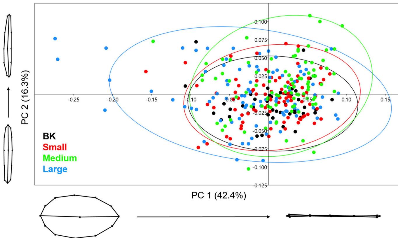
Fig. 6. Scatter plot of the PCA results comparing the morphological shapes of BK cut marks with the three main quartzite size groups (small, medium and large) in shape space. Extreme shape changes can be observed across the axis of each PC score.
